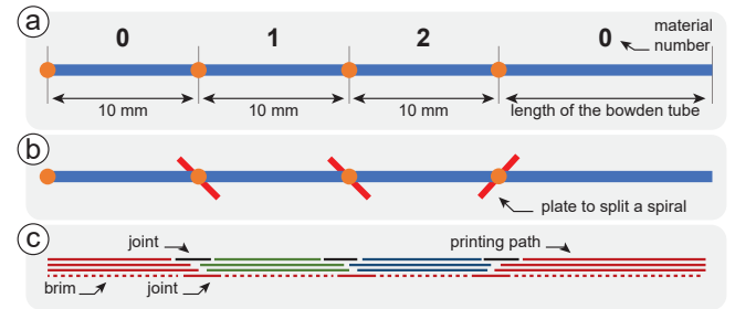
Figure 8. Process of the filament generation, with example input of length = 10, 10, 10 and material = 0, 1, 2 . The software generates a spiral then (a) labels each segment, (b) splits the spiral into segments using cutting-planes, and (c) generates a G-code of the filament for each layer.
