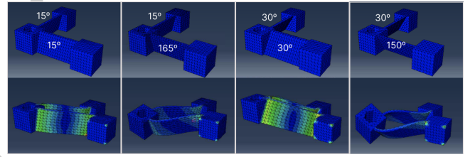
Figure 21: Representative simulations conducted in Abaqus
