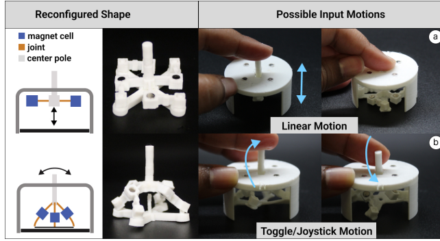
Figure 16: Push button motion (a) can be reconfigured to a toggle or joystick motion (b) by pulling up the center pole.
