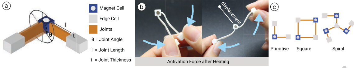
Figure 2: The structure of the shape-change geometry (a) is extracted from an elbow-joint building block. Geometric parameters program displacement of the magnet cell through shape change. Activation forces (b) are applied at the edge cells to bring them closer, or pull them apart in the same plane. We explore three topologies of the primitive (c).
