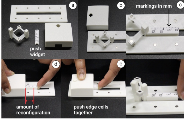
Figure 20: Using push widget for reconfiguration through pushing edge cells together
