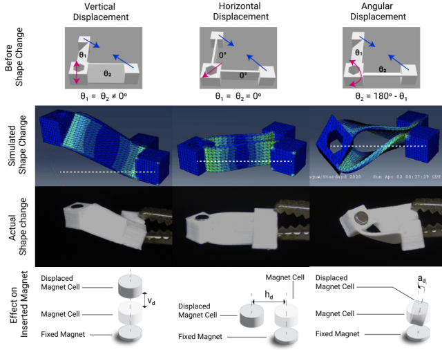
Figure 4: Vertical, Horizontal, and Angular displacement modules before/after shape change with their simulated models and the abstraction of the effect on embedded magnets.
