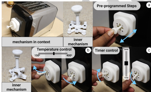
Figure 17: Push interface can activate a pre-programmed set of steps for toasting (a). Reconfiguration of the mechanism can enable full control over temperature (b) and timer (c) settings through a four-way toggle motion.
