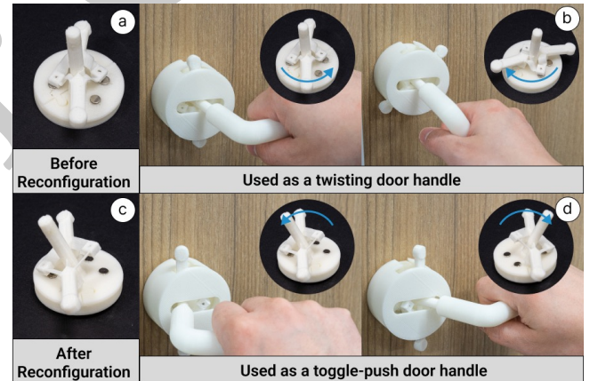
Figure 15: Reconfiguring twist motion (a,b) to toggle (c,d), afforded and constrained by shape change and magnets.
