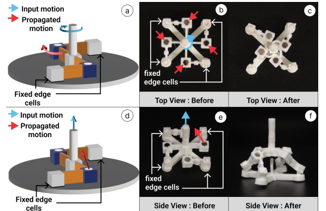
Figure 6: A spiral topology can utilize a center pole and stoppers, or even have its edge cells fixed (a,b). Rotation the pole results in magnets cells moving closer to the pole (c), and pulling up the pole (d,e) results in a dome shape (f)
