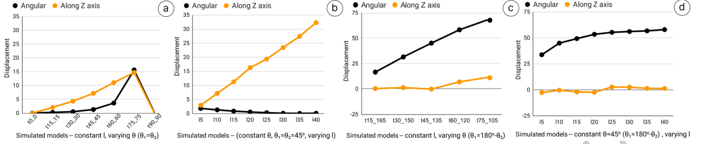
Figure 22: Displacements for (a) constant joint length ( l ) and increasing \theta_1 = \theta_2 , (b) constant joint angle ( \theta_1 = \theta_2 = 45^\circ ) and increasing joint lengths ( l ), (c) constant joint length ( l ) and increasing \theta_1 = 180^\circ - \theta_2 , (d) constant joint angle ( \theta_1 = 45^\circ, \theta_2 = 135^\circ ) and increasing joint lengths ( l ).
