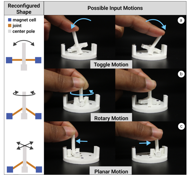
Figure 14: Reconfigured shape change enables reconfiguring toggle motion (a) to rotary motion (b) to planar motion (c).
