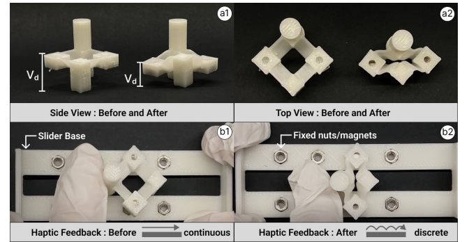
Figure 8: Vertical displacement of the magnet cells moves magnets closer to the slider base (a1,a2) increasing the feedback felt while moving the slider from a continuous motion with minimal feedback to discrete stepped feedback (b1,b2).
