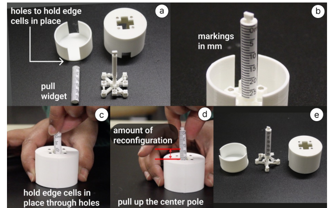
Figure 19: Using pull widget for reconfiguration through pulling up of center pole
