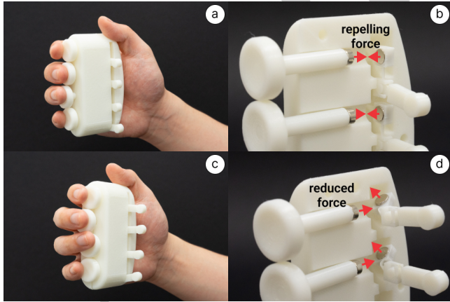
Figure 10: Re-orienting the aligned magnets of a rehabilitation device (a,b) reducing force feedback (c,d).
