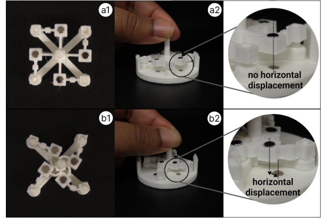
Figure 11: Twisting the central pole of the spiral (a) moves magnet cells close to the center in horizontal displacement (b) with the fixed base magnets, and changes received feedback.
