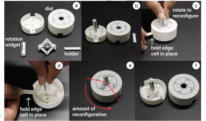
Figure 18: Using rotation widget for reconfiguration through rotation of center pole
